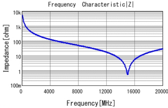
■ GJM1555C1HR30BB01 |Z| DC0V, 25degC
