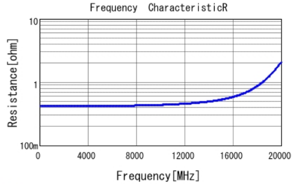
■ GJM1555C1HR30BB01 R DC0V, 25degC
