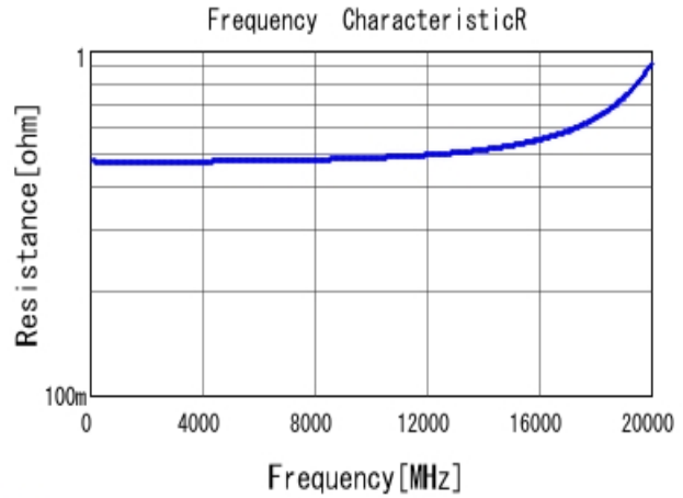
■ GJM1555C1HR20WB01 R DC0V, 25degC
