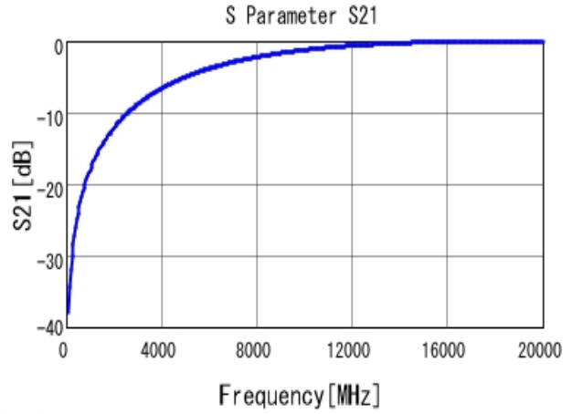
■ GJM1555C1HR20WB01 S21 DCOV, 25degC
