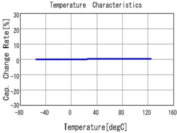
■ GJM1555C1HR20WB01 C-Temp. capchange, DCOV, AC1Vrms
