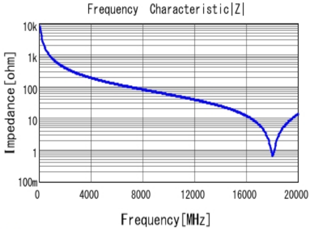
■ GJM1555C1HR20WB01 |Z| DC0V, 25degC
