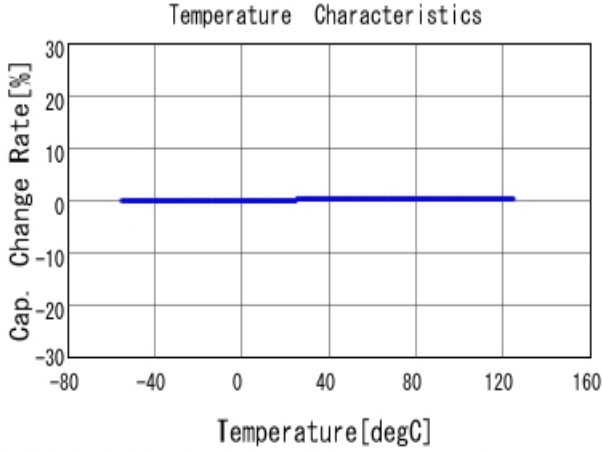
■ GJM1555C1HR10WB01 C-Temp. capchange, DCOV, AC1Vrms
