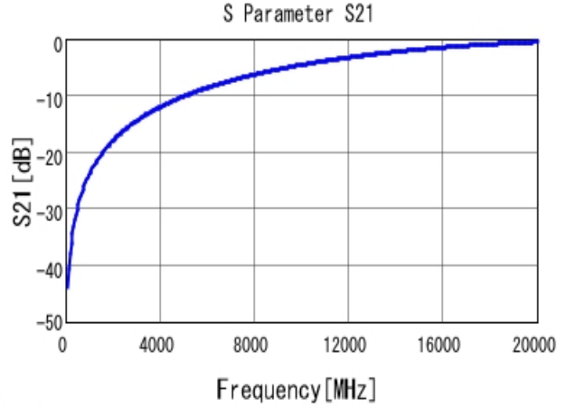
■ GJM1555C1HR10WB01 S21 DCOV, 25degC
