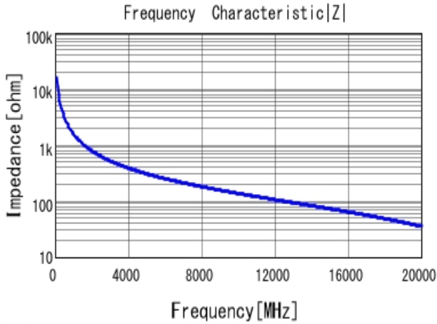
GJM1555C1HR10WB01 |Z| DC0V, 25degC
