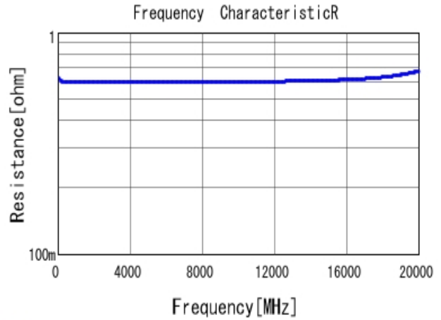
GJM1555C1HR10WB01 R DC0V, 25degC
