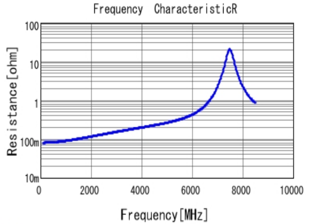
■ GJM1555C1H9R1CB01 R DC0V, 25degC
