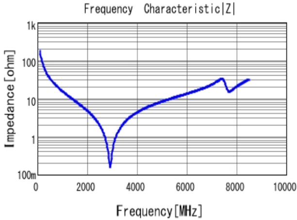
■ GJM1555C1H9R1CB01 |Z| DC0V, 25degC
