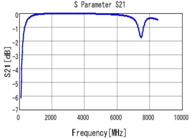
■ GJM1555C1H9R0DB01 S21 DCOV, 25degC
