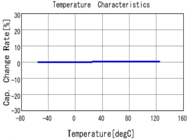
■ GJM1555C1H9R0DB01 C-Temp. capchange, DCOV, AC1Vrms
