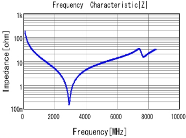
■ GJM1555C1H9R0DB01 |Z| DC0V, 25degC
