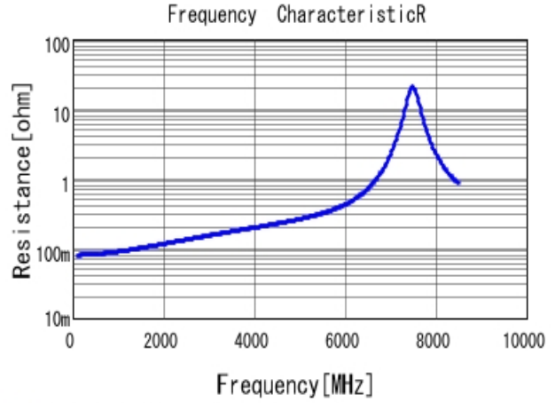
■ GJM1555C1H9R0DB01 R DC0V, 25degC
