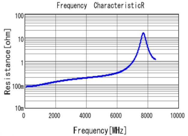
■ GJM1555C1H8R2WB01 R DC0V, 25degC
