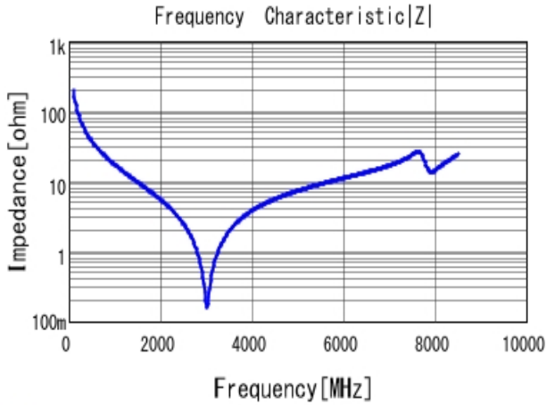
■ GJM1555C1H8R2WB01 |Z| DC0V, 25degC
