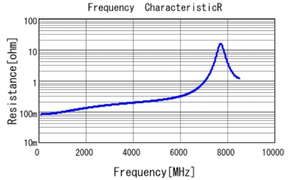
■ GJM1555C1H8R2BB01 R DC0V, 25degC
