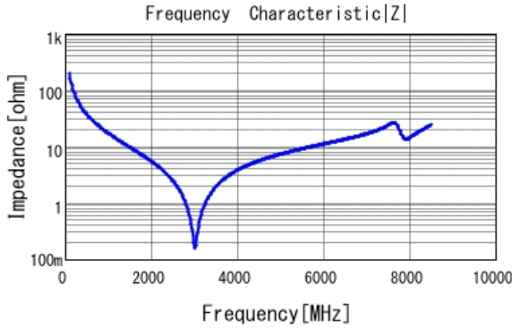
■ GJM1555C1H8R2BB01 |Z| DC0V, 25degC
