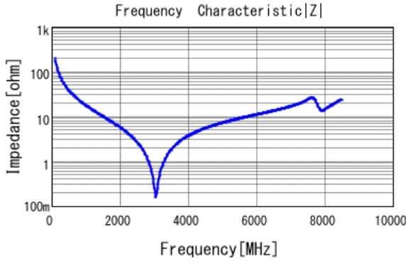
■ GJM1555C1H8R0CB01 |Z| DCOV, 25degC
