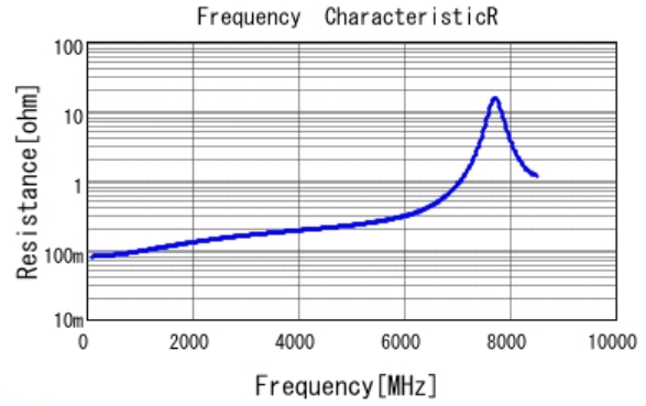
■ GJM1555C1H8R0CB01 R DCOV, 25degC
