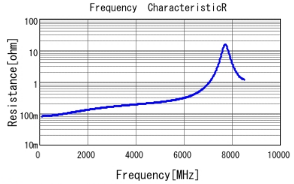
■ GJM1555C1H8R0BB01 R DCOV, 25degC
