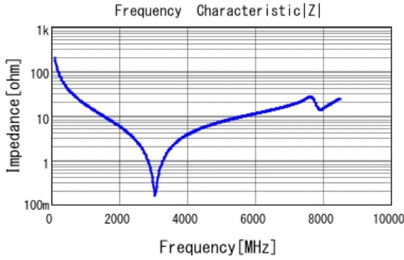
■ GJM1555C1H8R0BB01 |Z| DCOV, 25degC
