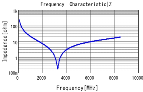
■ GJM1555C1H6R8BB01 |Z| DCOV, 25degC
