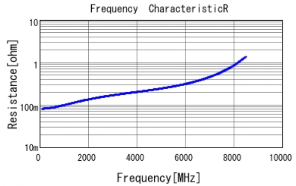
■ GJM1555C1H6R8BB01 R DCOV, 25degC
