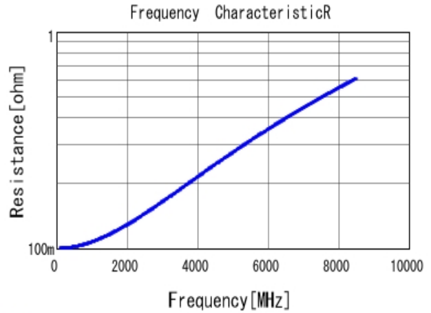
■ GJM1555C1H5R6CB01 R DC0V, 25degC
