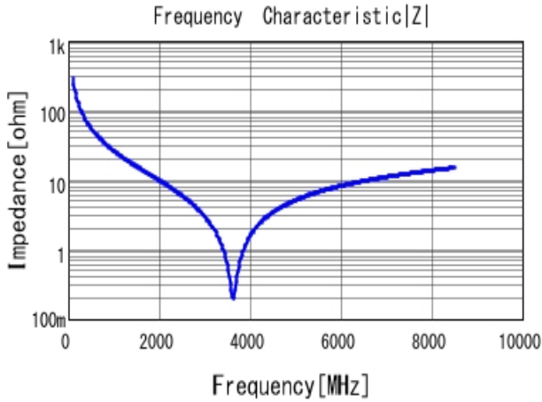
■ GJM1555C1H5R6CB01 |Z| DC0V, 25degC
