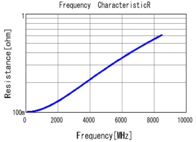
GJM1555C1H5R6BB01 R DC0V, 25degC
