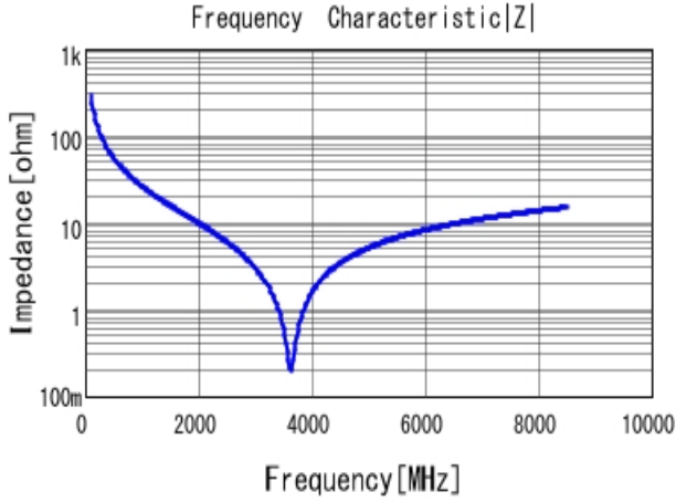
GJM1555C1H5R6BB01 |Z| DC0V, 25degC
