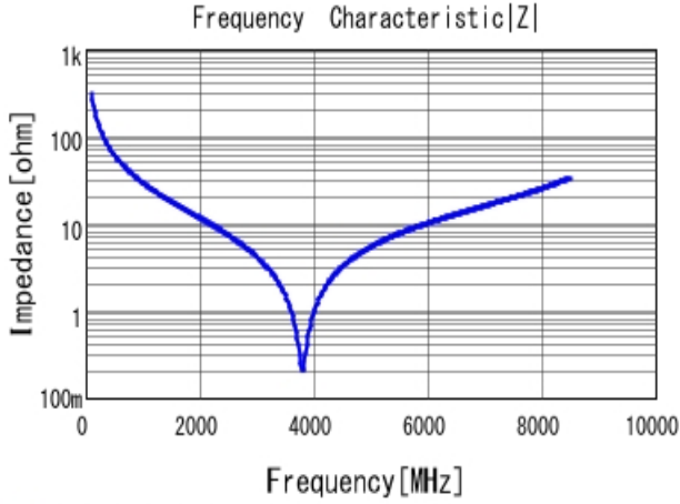
GJM1555C1H5R1WB01 |Z| DC0V, 25degC
