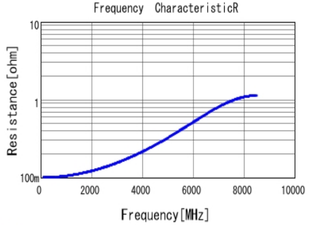
GJM1555C1H5R1WB01 R DC0V, 25degC
