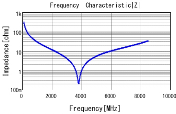
■ GJM1555C1H5R1BB01 |Z| DC0V, 25degC
