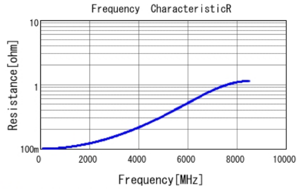
■ GJM1555C1H5R1BB01 R DC0V, 25degC
