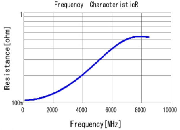
■ GJM1555C1H4R7BB01 R DC0V, 25degC
