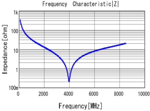
■ GJM1555C1H4R7BB01 |Z| DC0V, 25degC
