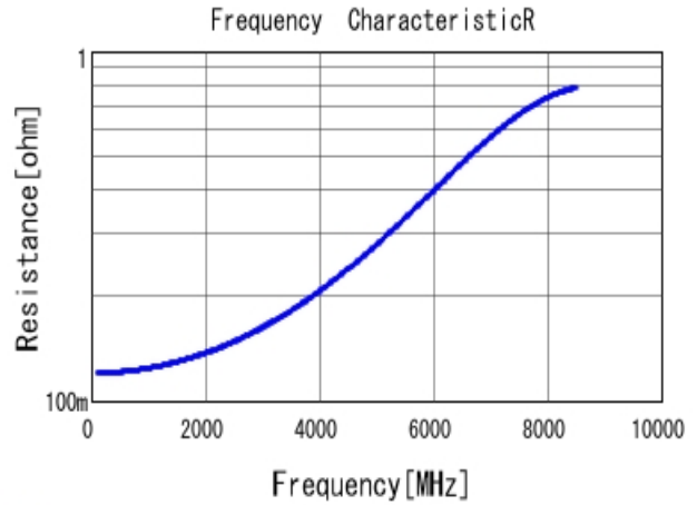
■ GJM1555C1H3R9CB01 R DC0V, 25degC
