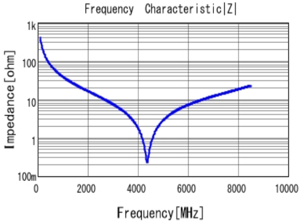
■ GJM1555C1H3R9CB01 |Z| DC0V, 25degC
