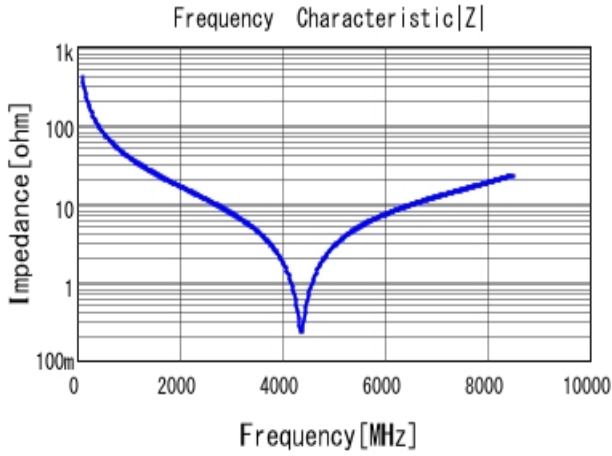
■ GJM1555C1H3R9BB01 |Z| DC0V, 25degC
