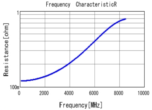
■ GJM1555C1H3R9BB01 R DC0V, 25degC
