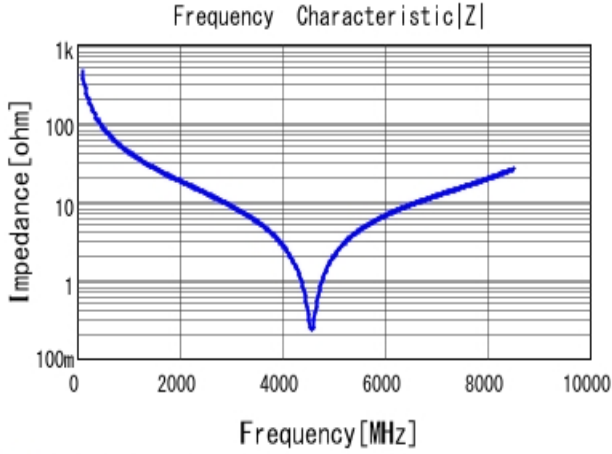
GJM1555C1H3R6WB01 |Z| DC0V, 25degC
