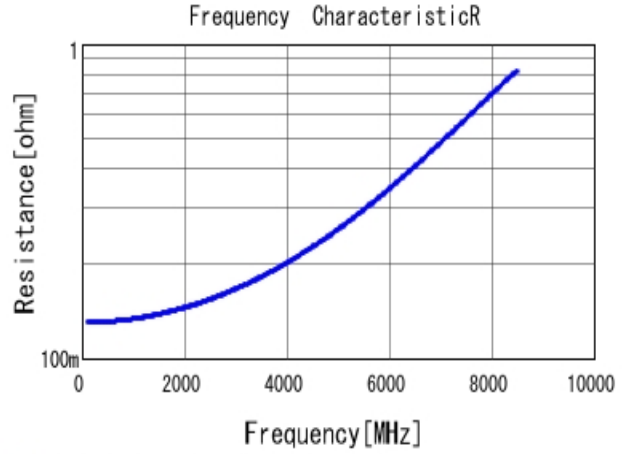
GJM1555C1H3R6WB01 R DC0V, 25degC
