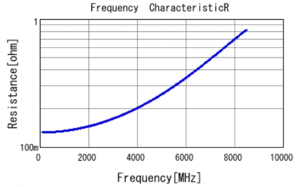
■ GJM1555C1H3R6CB01 R DC0V, 25degC
