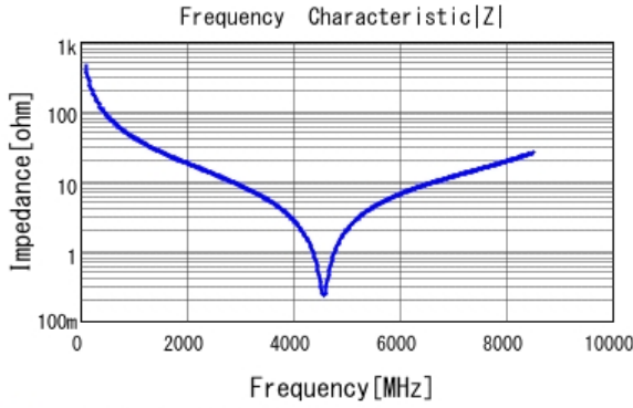
■ GJM1555C1H3R6CB01 |Z| DC0V, 25degC
