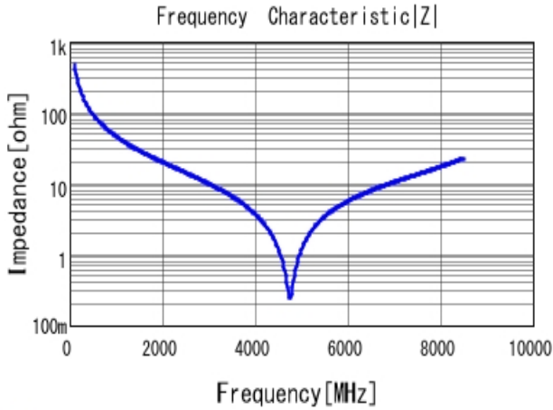
GJM1555C1H3R3BB01 |Z| DC0V, 25degC
