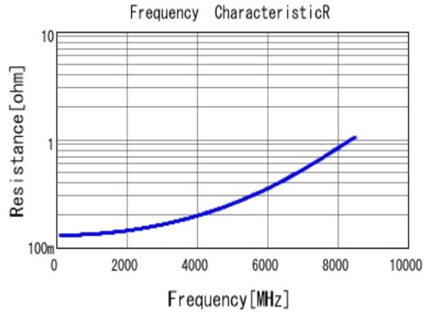
GJM1555C1H3R3BB01 R DC0V, 25degC
