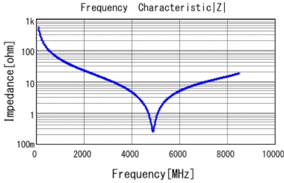
■ GJM1555C1H3R0WB01 |Z| DCOV, 25degC
