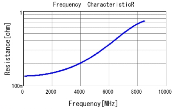
■ GJM1555C1H3R0WB01 R DCOV, 25degC
