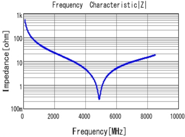
GJM1555C1H3R0CB01 |Z| DC0V, 25degC
