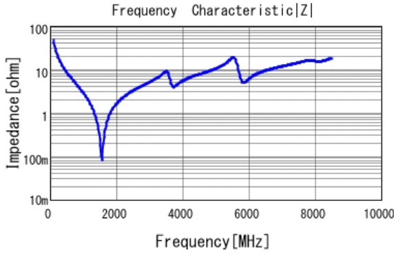
■ GJM1555C1H330FB01 |Z| DC0V, 25degC
