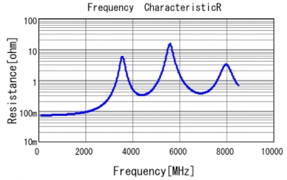
■ GJM1555C1H330FB01 R DC0V, 25degC
