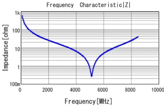
■ GJM1555C1H2R7CB01 |Z| DC0V, 25degC
