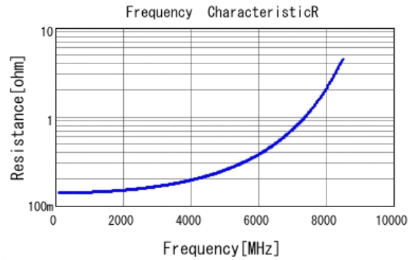
■ GJM1555C1H2R7CB01 R DC0V, 25degC
