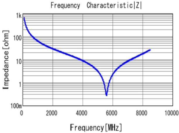
GJM1555C1H2R4CB01 |Z| DC0V, 25degC
