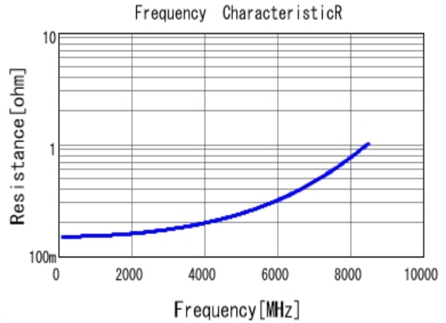
GJM1555C1H2R4CB01 R DC0V, 25degC
