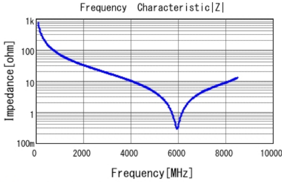
■ GJM1555C1H2R2WB01 |Z| DC0V, 25degC
