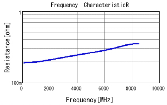
■ GJM1555C1H2R0BB01 R DC0V, 25degC
