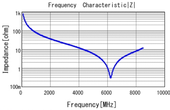
■ GJM1555C1H2R0BB01 |Z| DC0V, 25degC
