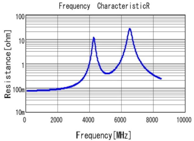
■ GJM1555C1H220FB01 R DCOV, 25degC
