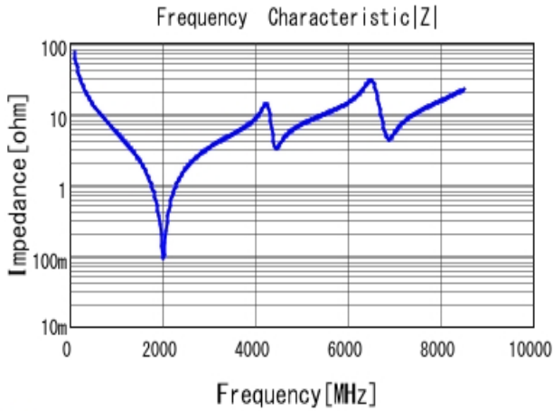
■ GJM1555C1H220FB01 |Z| DCOV, 25degC
