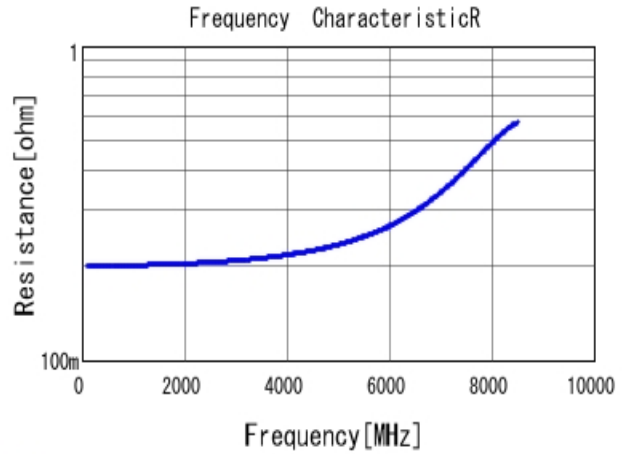
■ GJM1555C1H1R9WB01 R DC0V, 25degC
