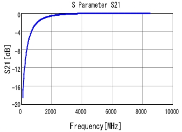
■ GJM1555C1H1R9WB01 S21 DCOV, 25degC
