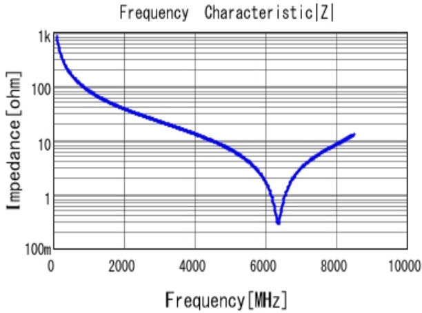
■ GJM1555C1H1R9WB01 |Z| DC0V, 25degC
