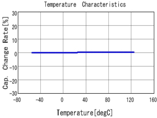
■ GJM1555C1H1R9WB01 C-Temp. capchange, DCOV, AC1Vrms
