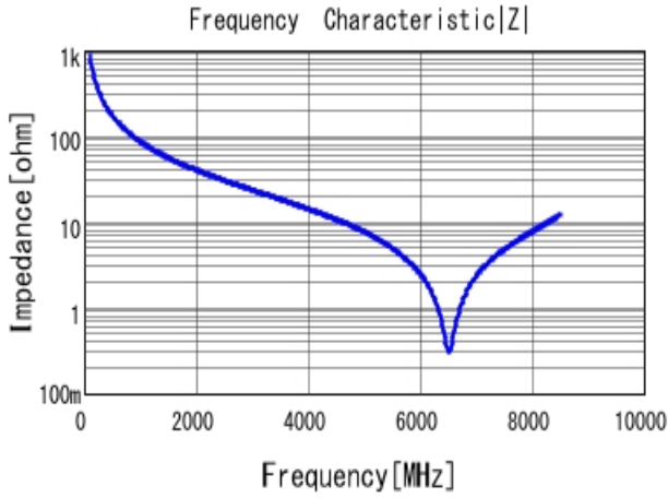
■ GJM1555C1H1R8BB01 |Z| DC0V, 25degC
