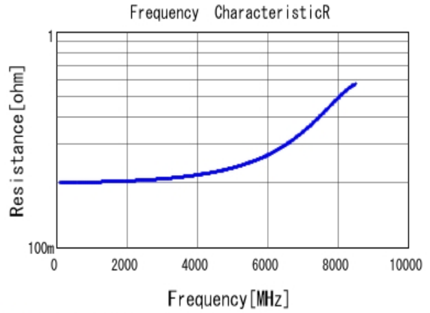
■ GJM1555C1H1R8BB01 R DC0V, 25degC
