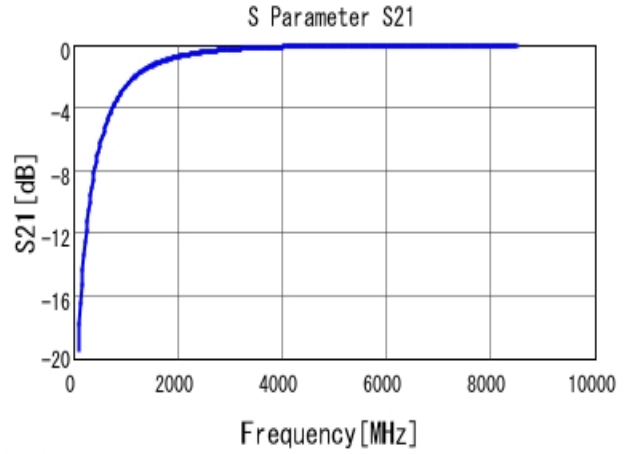
■ GJM1555C1H1R7WB01 S21 DCOV, 25degC
