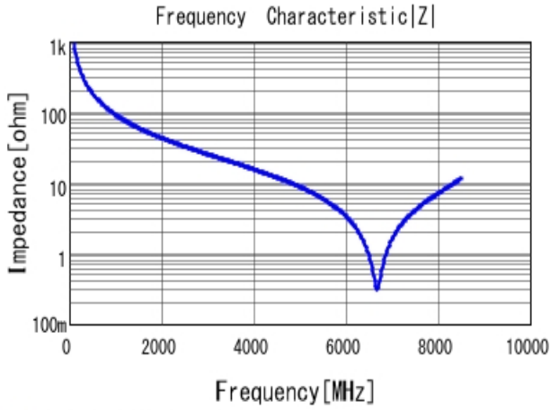
■ GJM1555C1H1R7WB01 |Z| DC0V, 25degC
