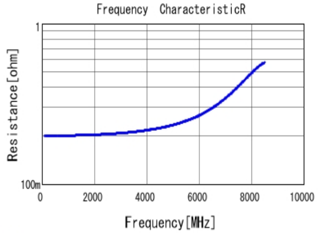
■ GJM1555C1H1R7WB01 R DC0V, 25degC
