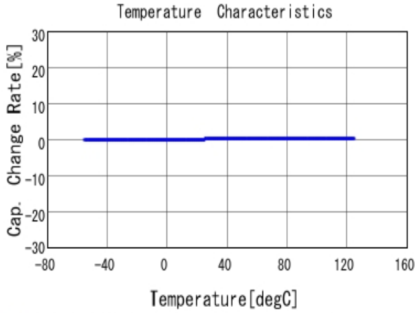
■ GJM1555C1H1R7WB01 C-Temp. capchange, DCOV, AC1Vrms
