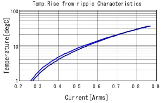
GJM1555C1H1R5BB01 Temp. rise — 2GHz — 3GHz
