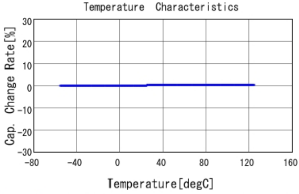
GJM1555C1H1R5BB01 C-Temp. capchange, DCOV, AC1Vrms
