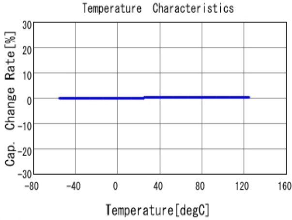
■ GJM1555C1H1R0WB01 C-Temp. capchange, DCOV, AC1Vrms
