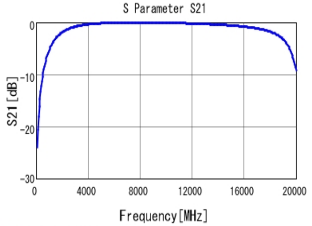
■ GJM1555C1H1R0WB01 S21 DCOV, 25degC
