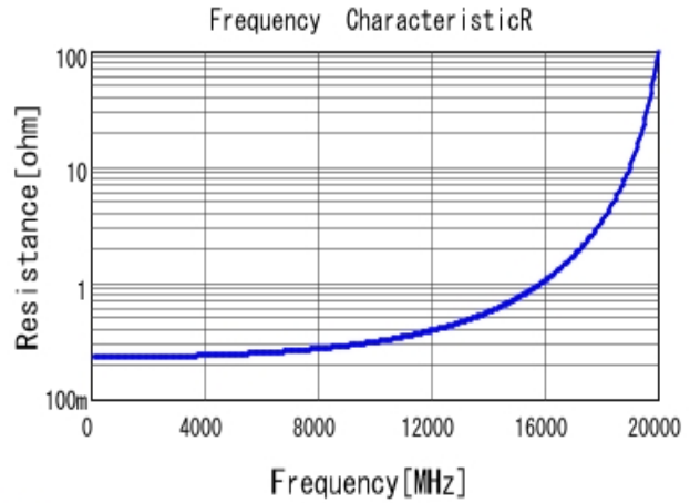
■ GJM1555C1H1R0WB01 R DC0V, 25degC
