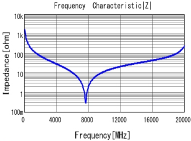
■ GJM1555C1H1R0WB01 |Z| DC0V, 25degC
