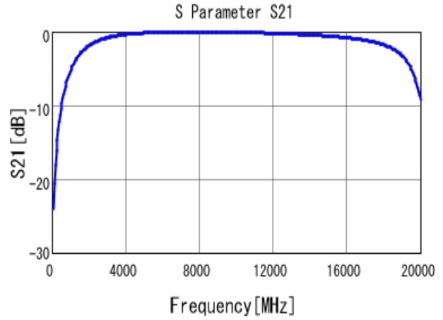
■ GJM1555C1H1R0CB01 S21 DCOV, 25degC
