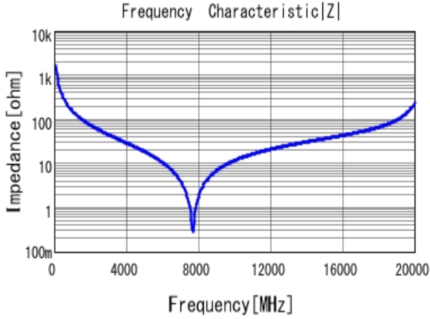
■ GJM1555C1H1R0CB01 |Z| DC0V, 25degC
