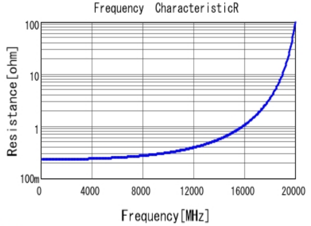
■ GJM1555C1H1R0CB01 R DC0V, 25degC
