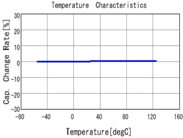
■ GJM1555C1H1R0CB01 C-Temp. capchange, DCOV, AC1Vrms
