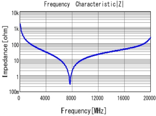
GJM1555C1H1R0BB01 |Z| DC0V, 25degC
