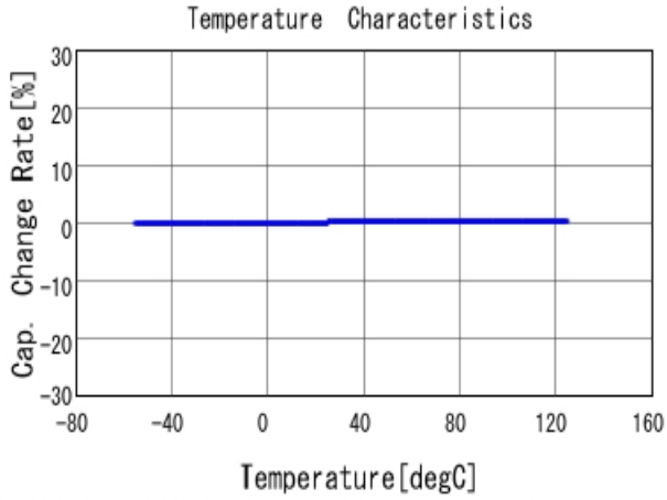
■ GJM1555C1H1R0BB01 C-Temp. capchange, DCOV, AC1Vrms
