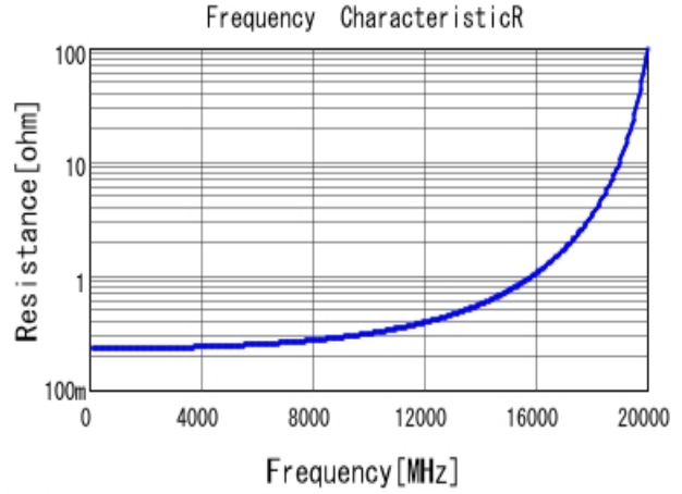
GJM1555C1H1R0BB01 R DC0V, 25degC
