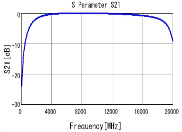
■ GJM1555C1H1R0BB01 S21 DCOV, 25degC
