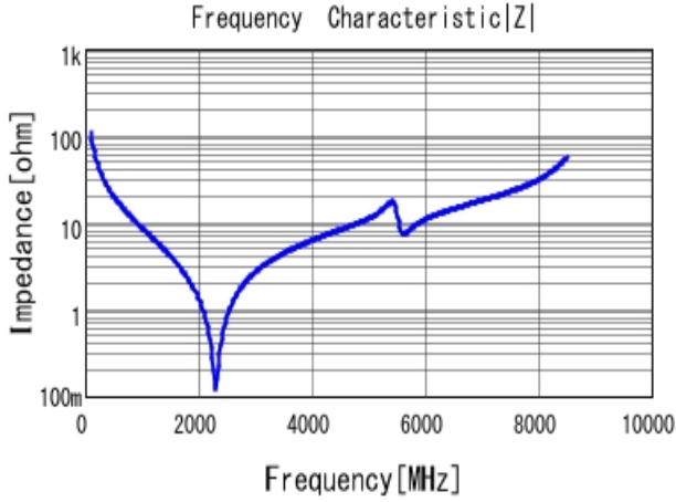
■ GJM1555C1H150JB01 |Z| DC0V, 25degC
