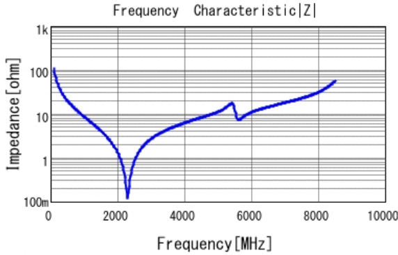
■ GJM1555C1H150FB01 |Z| DC0V, 25degC
