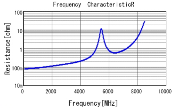
■ GJM1555C1H150FB01 R DC0V, 25degC
