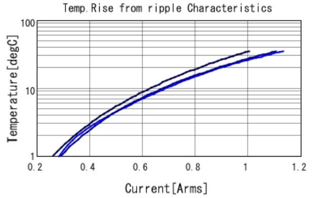
GJM1555C1H100FB01 Temp. rise — 700MHz — 1GHz
