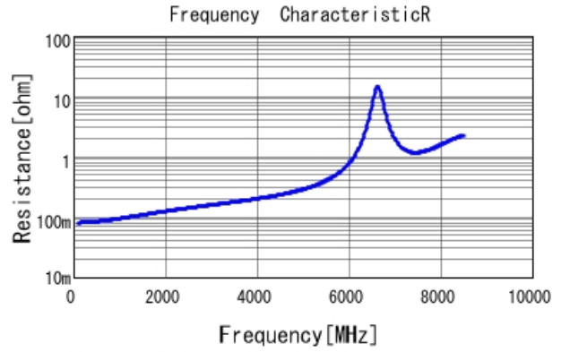
GJM1555C1H100FB01 R DCOV, 25degC
