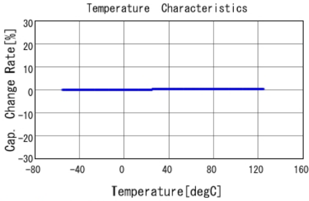
GJM1555C1H100FB01 C-Temp. capchange, DCOV, AC1Vrms
