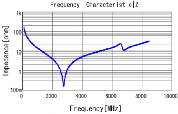
GJM1555C1H100FB01 |Z| DCOV, 25degC
