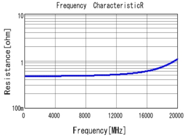
GJM0335C1HR40WB01 R DC0V, 25degC
