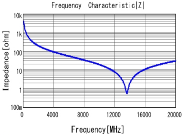
GJM0335C1HR40WB01 |Z| DC0V, 25degC
