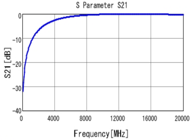
■ GJM0335C1HR40WB01 S21 DCOV, 25degC
