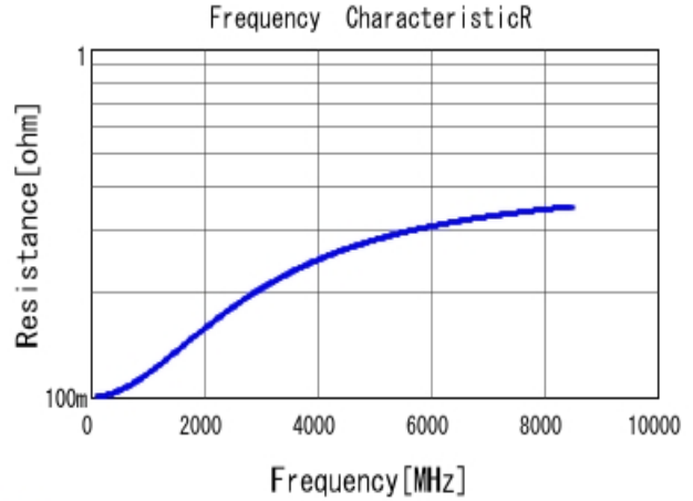
GJM0335C1E6R8BB01 R DC0V, 25degC
