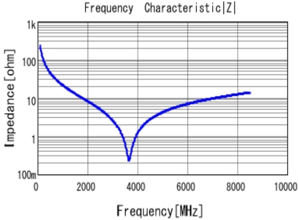
GJM0335C1E6R8BB01 |Z| DC0V, 25degC
