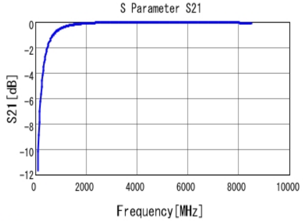
■ GJM0335C1E4R3BB01 S21 DCOV, 25degC
