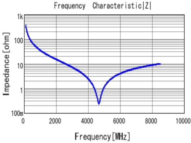
GJM0335C1E4R3BB01 |Z| DC0V, 25degC
