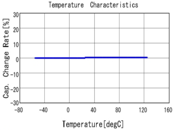
■ GJM0335C1E4R3BB01 C-Temp. capchange, DCOV, AC1Vrms
