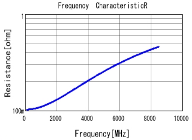
GJM0335C1E4R3BB01 R DC0V, 25degC
