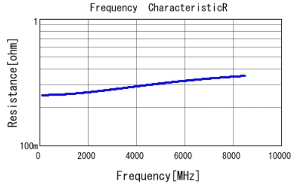
■ GJM0335C1E1R5CB01 R DC0V, 25degC
