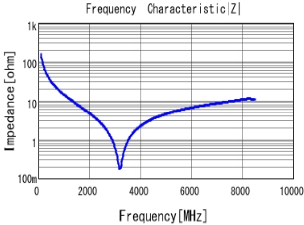
GJM0335C1E100GB01 |Z| DC0V, 25degC
