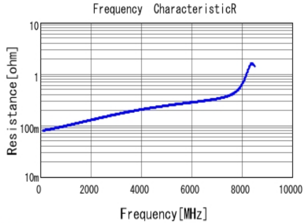
GJM0335C1E100GB01 R DC0V, 25degC
