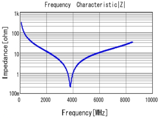
■ GCQ1555C1H5R1BB01 |Z| DC0V, 25degC
