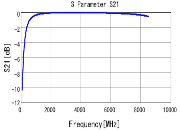
■ GCQ1555C1H5R1BB01 S21 DCOV, 25degC
