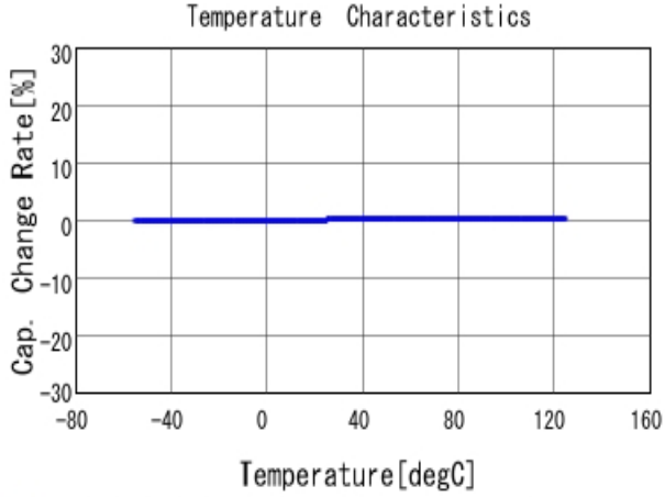
■ GCQ1555C1H5R1BB01 C-Temp. capchange, DCOV, AC1Vrms
