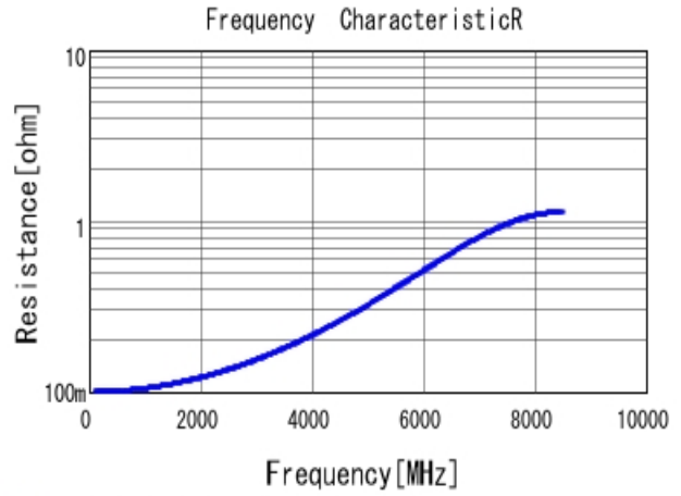
■ GCQ1555C1H5R1BB01 R DC0V, 25degC
