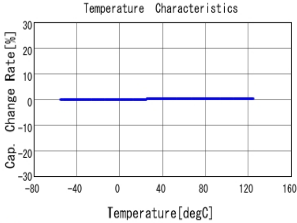
■ GCQ1555C1H4R3CB01 C-Temp. capchange, DCOV, AC1Vrms
