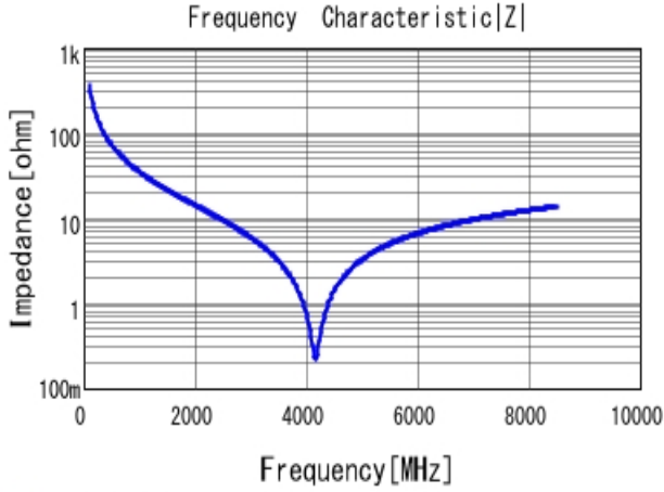
■ GCQ1555C1H4R3CB01 |Z| DC0V, 25degC
