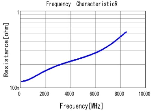
■ GCQ1555C1H4R3CB01 R DC0V, 25degC
