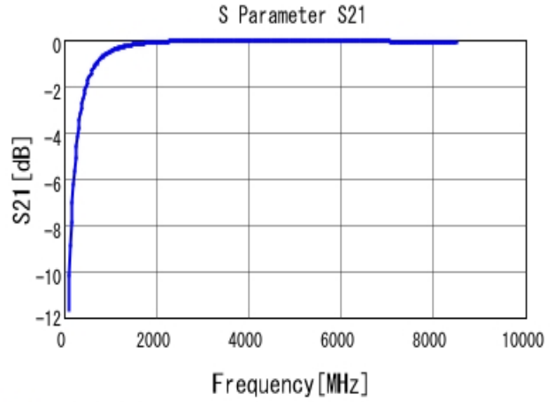
■ GCQ1555C1H4R3CB01 S21 DCOV, 25degC
