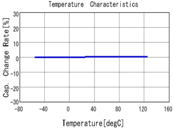
■ GCQ1555C1H470JB01 C-Temp. capchange, DCOV, AC1Vrms
