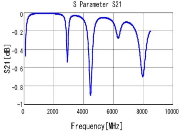
■ GCQ1555C1H470JB01 S21 DCOV, 25degC
