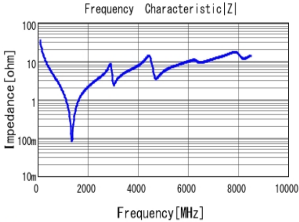
■ GCQ1555C1H470JB01 |Z| DC0V, 25degC
