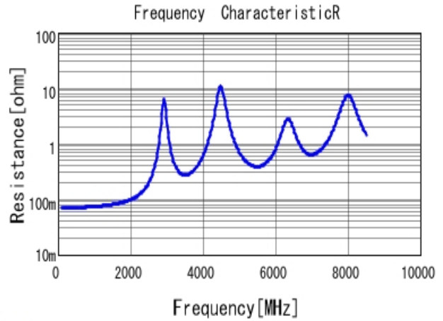
■ GCQ1555C1H470JB01 R DC0V, 25degC
