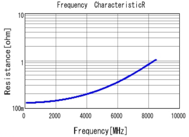
■ GCQ1555C1H3R3BB01 R DC0V, 25degC
