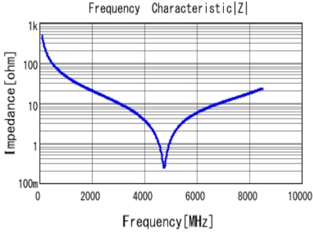
■ GCQ1555C1H3R3BB01 |Z| DC0V, 25degC
