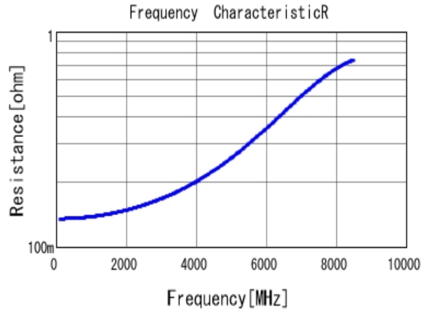
■ GCQ1555C1H3R0WB01 R DC0V, 25degC
