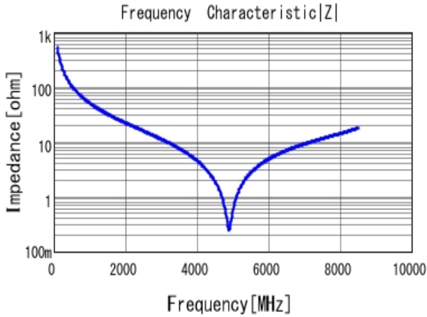
■ GCQ1555C1H3R0WB01 |Z| DC0V, 25degC
