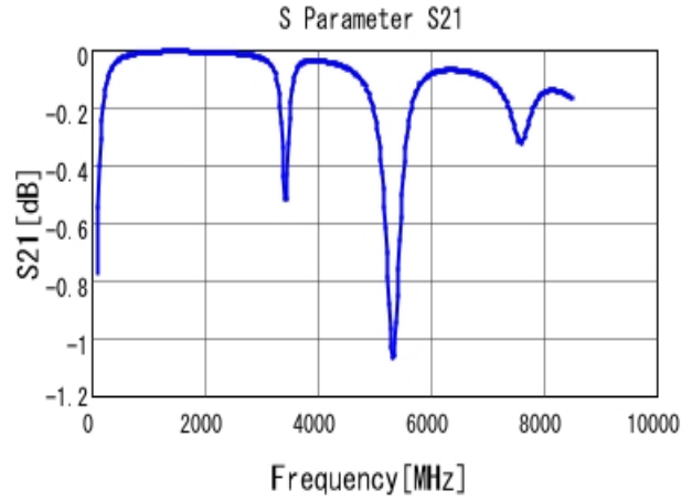
■ GCQ1555C1H360JB01 S21 DCOV, 25degC
