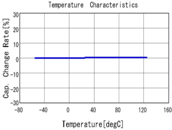
■ GCQ1555C1H360JB01 C-Temp. capchange, DCOV, AC1Vrms
