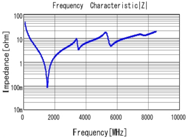
■ GCQ1555C1H360JB01 |Z| DC0V, 25degC
