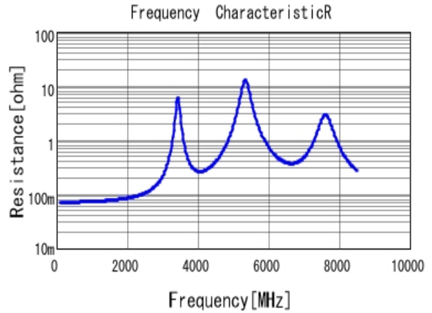
■ GCQ1555C1H360JB01 R DC0V, 25degC
