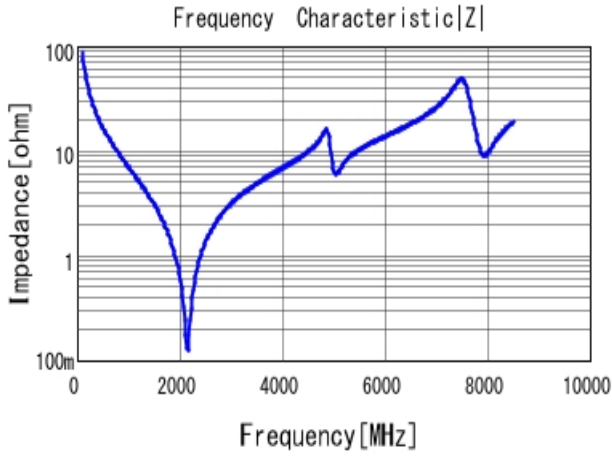
■ GCQ1555C1H180GB01 |Z| DC0V, 25degC
