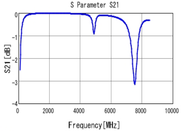
■ GCQ1555C1H180GB01 S21 DCOV, 25degC
