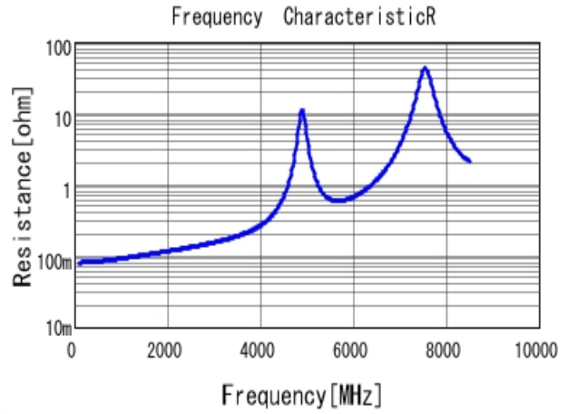
■ GCQ1555C1H180GB01 R DC0V, 25degC
