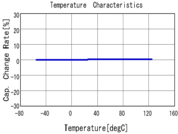
■ GCQ1555C1H180GB01 C-Temp. capchange, DCOV, AC1Vrms
